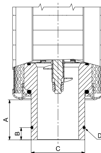
Fig. 68 Suction pipe
