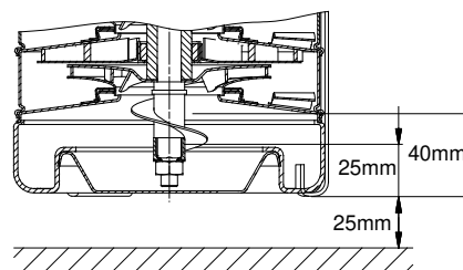
Fig. 27 Minimum distance between pump and tank
