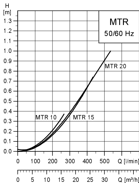
Fig. 46 Pressure losses of pumped liquid passing through an empty chamber for MTR 10, MTR 15 and MTR 20 pumps
