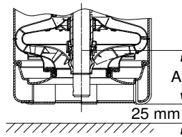
Fig. 23 MTR, MTRE 32, 45 and 64
