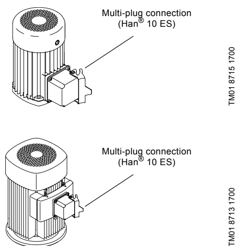
Fig. 32 Multi-plug on a Grundfos MG motor
