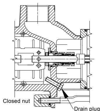
Fig. 67 Horizontal installation
