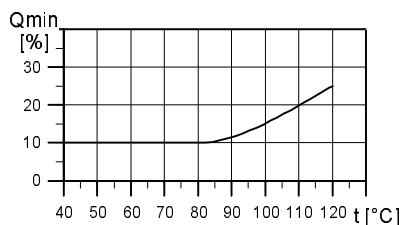
Fig. 56 Minimum flow rate
