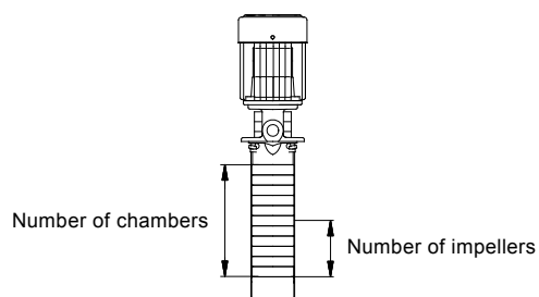
Fig. 15 MTR pump
