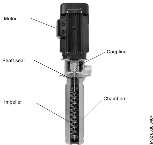
Fig. 3 MTR pump
