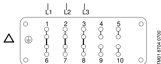
Fig. 37 Plug connections for delta connection. Fishplates for connections are located in the plug.
