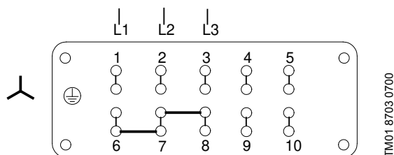
Fig. 36 Plug connections for star connection
