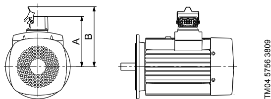
Fig. 34 Motor with multi-plug
