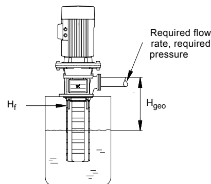
Fig. 41 Dimensional data
