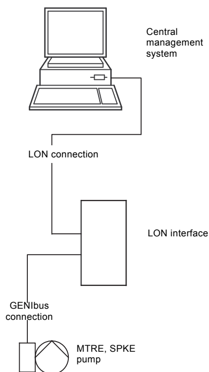
Fig. 52 Example of a central management system with LON interface
