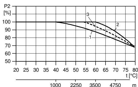
Fig. 8 The maximum motor output depends on the ambient temperature/altitude.
