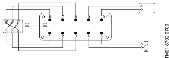
Fig. 35 From motor
