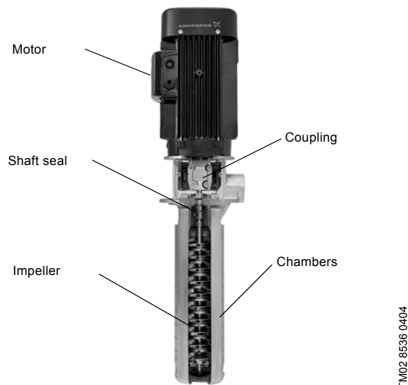
Fig. 4 SPK pump
